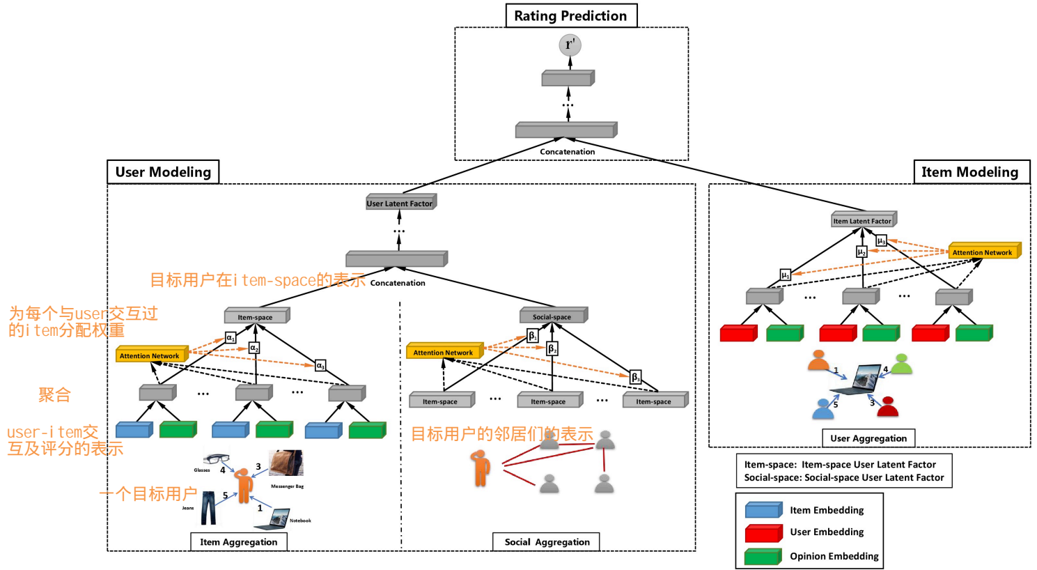
Figure 2: The overall architecture of the proposed model. It contains three major components: user modeling, item modeling, and rating prediction.
